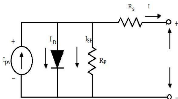
Figure 1.2 Single Diode Mathematic Model of PV Cell
