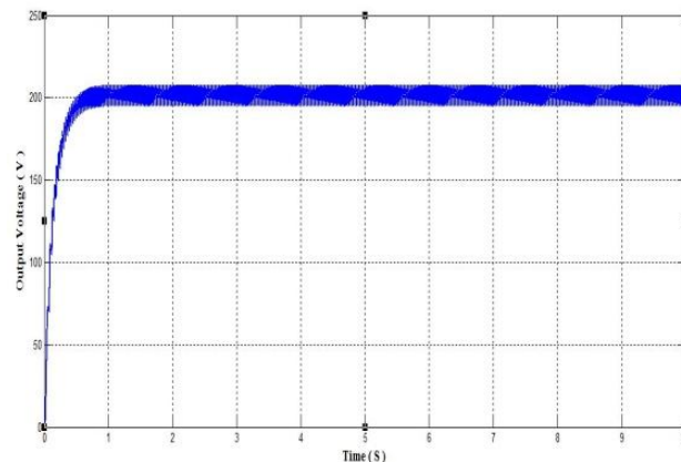
Figure 3.2 The Input Voltage Waveform of Neural Network Based MPPT Technique
