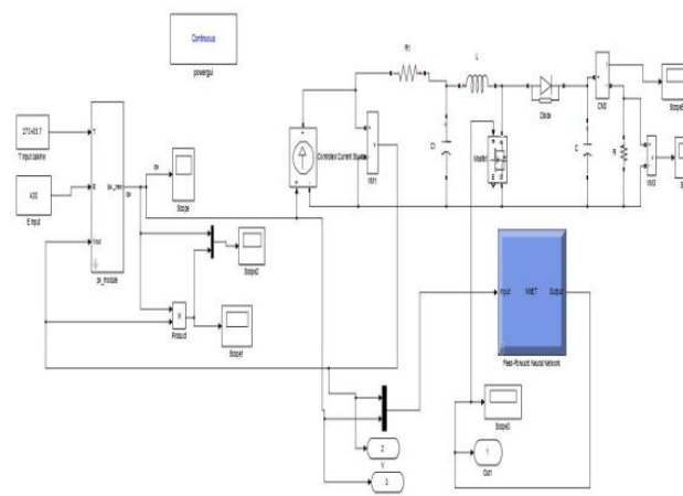
Figure 3.3 Simulation Model in Neural Network-Based-
