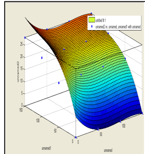
Fig. 2. A bi-cubic Bezier Surface.
